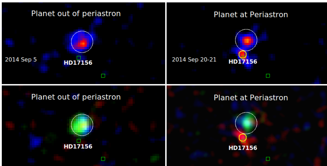
Figure 1. X-ray images of HD 17156 taken far from the planetary periastron (left side panels) and near the periastron (right side panels). Top row panels are intensity images, bottom row panels are RGB images with photon energy colors R = 0.3 - 1.0 keV, G = 1.0 - 2.5 keV, B = 2.5 - 5.0 keV. Smoothing is applied to the images, with a Gaussian of \sigma = 2.4'' for the intensity images and \sigma = 4'' for the RGB images. Positions of the only two objects in the SIMBAD catalog are shown with small squares. Circle sizes indicate the wavelet detection scales of HD 17156 and of an unrelated background object with an harder spectrum.
